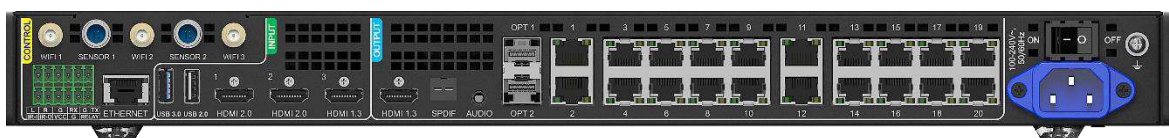
Figure 3-2 Rear panel – TU4K Pro (20 Ethernet ports)
