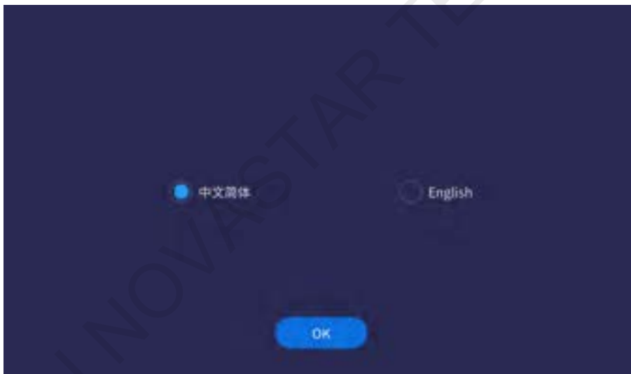
Figure 5-11 Web page
