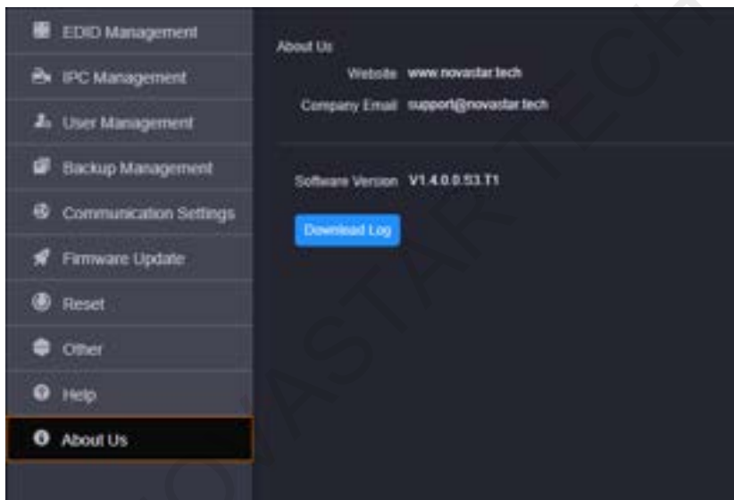
Figure 6-31 About us
