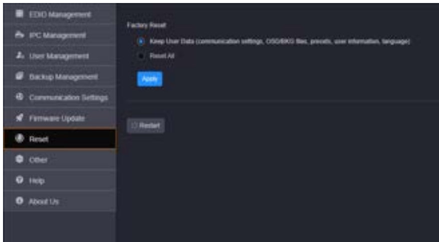
Figure 6-27 Reset
