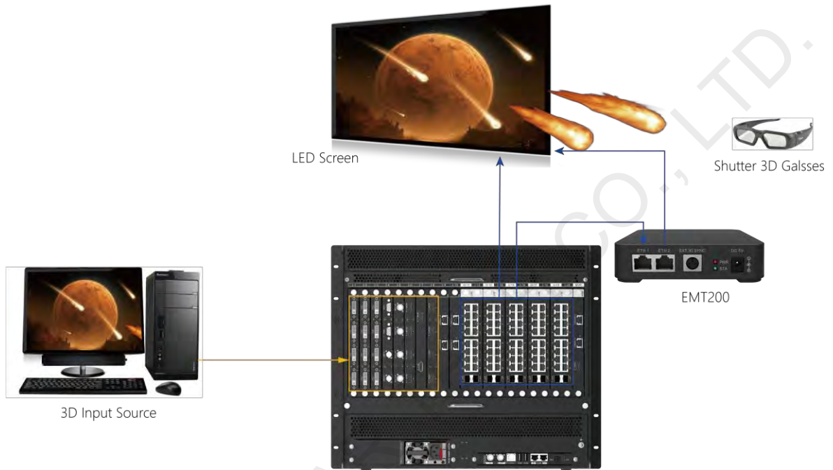
Figure 4-21 Hardware connections
