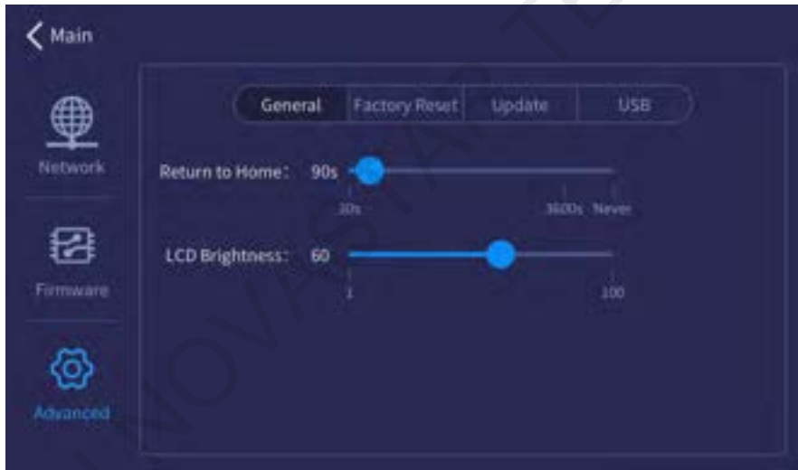
Figure 5-8 Advanced settings
