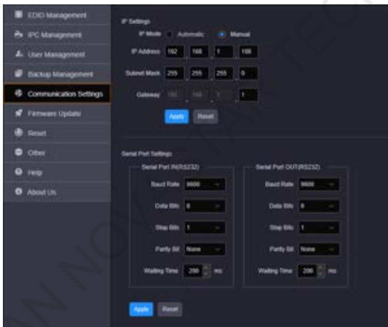
Figure 6-25 Communication settings
