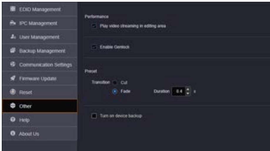
Figure 6-29 Other settings
