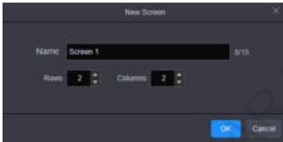
Figure 3-1 New screen
