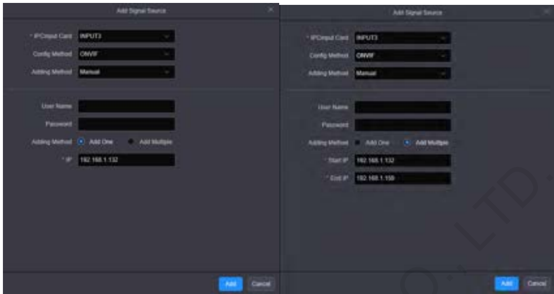
Figure 6-16 Adding manually
