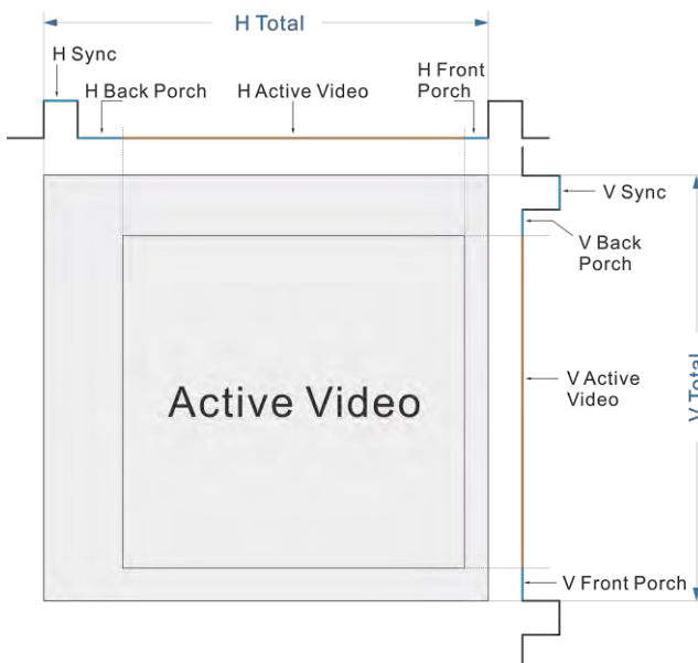
Figure 6-11 EDID management
