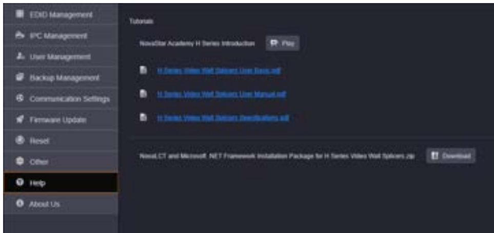
Figure 6-30 Help
