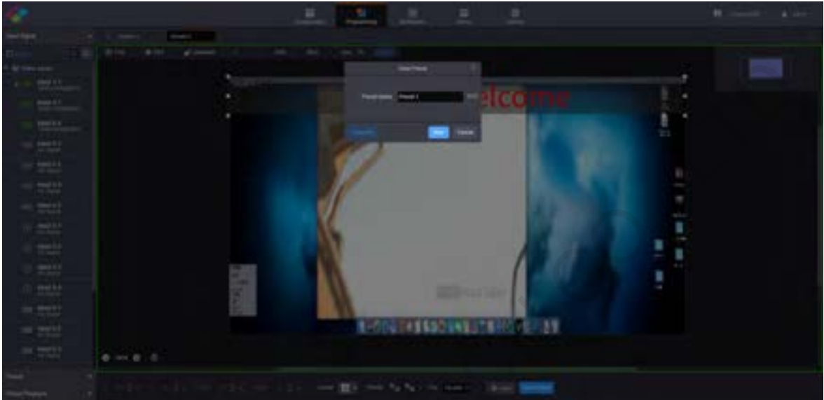
Figure 4-10 Saving presets
