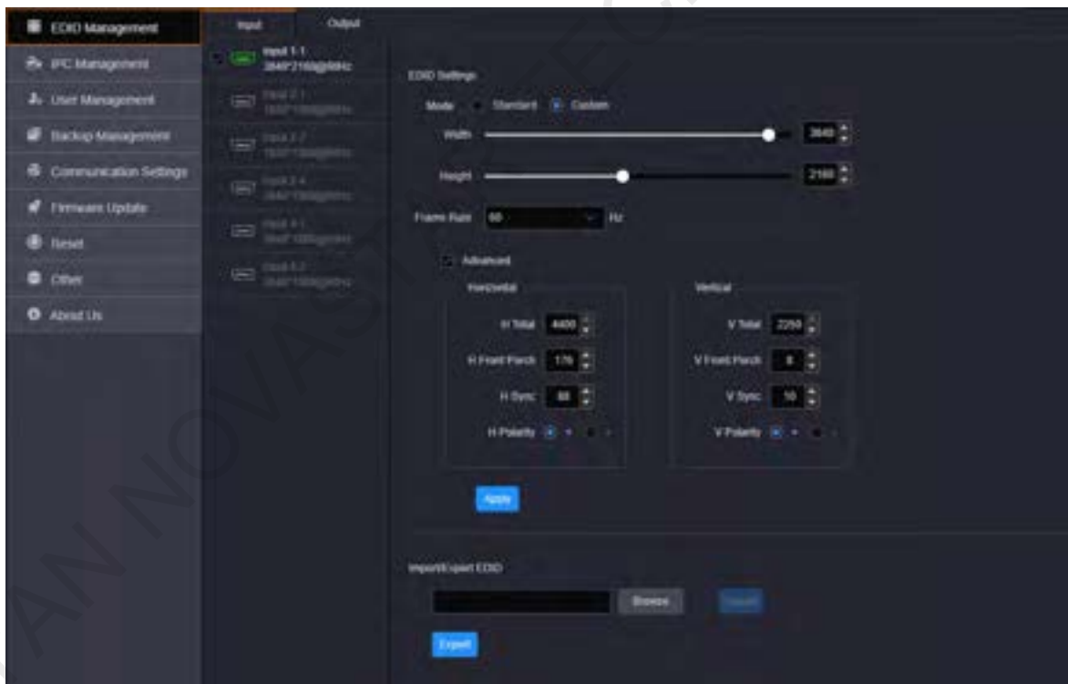
Figure 6-10 Settings
