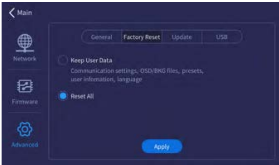
Figure 5-9 Factory reset
