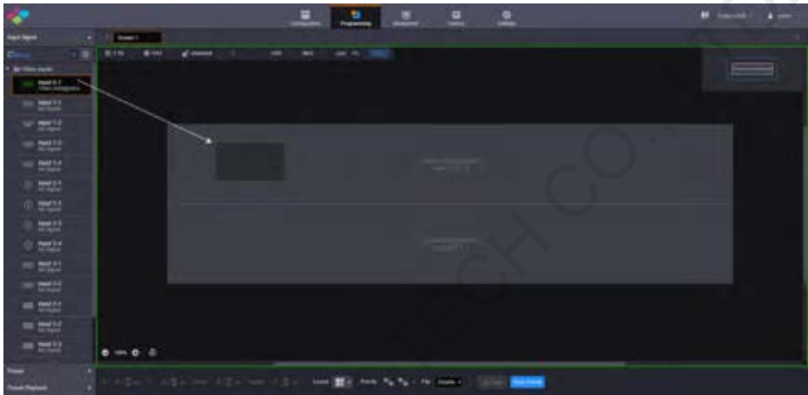
Figure 4-1 Adding layers
