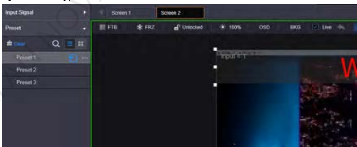
Figure 4-11 Loading presets
