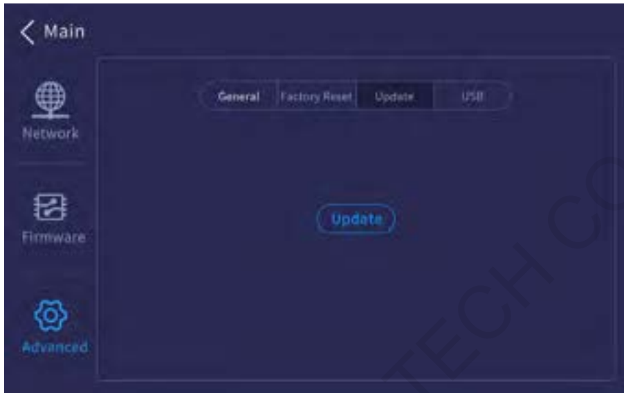
Figure 5-12 Firmware update
