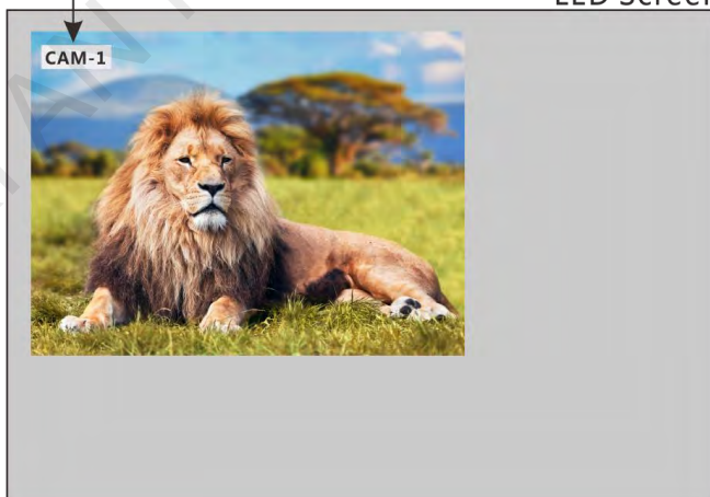
Figure 4-24 Channel logo
