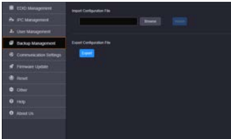
Figure 6-24 Backup management
